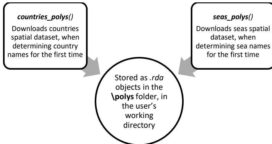
Figure 2. Functions for downloading the spatial datasets
