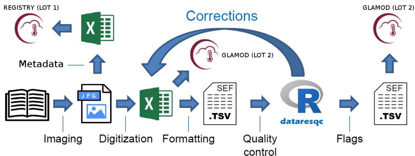
Figure 1. Workflow scheme illustrating all the steps to be taken for an efficient and traceable climate data and metadata transference from unusable formats to machine-readable data and metadata
